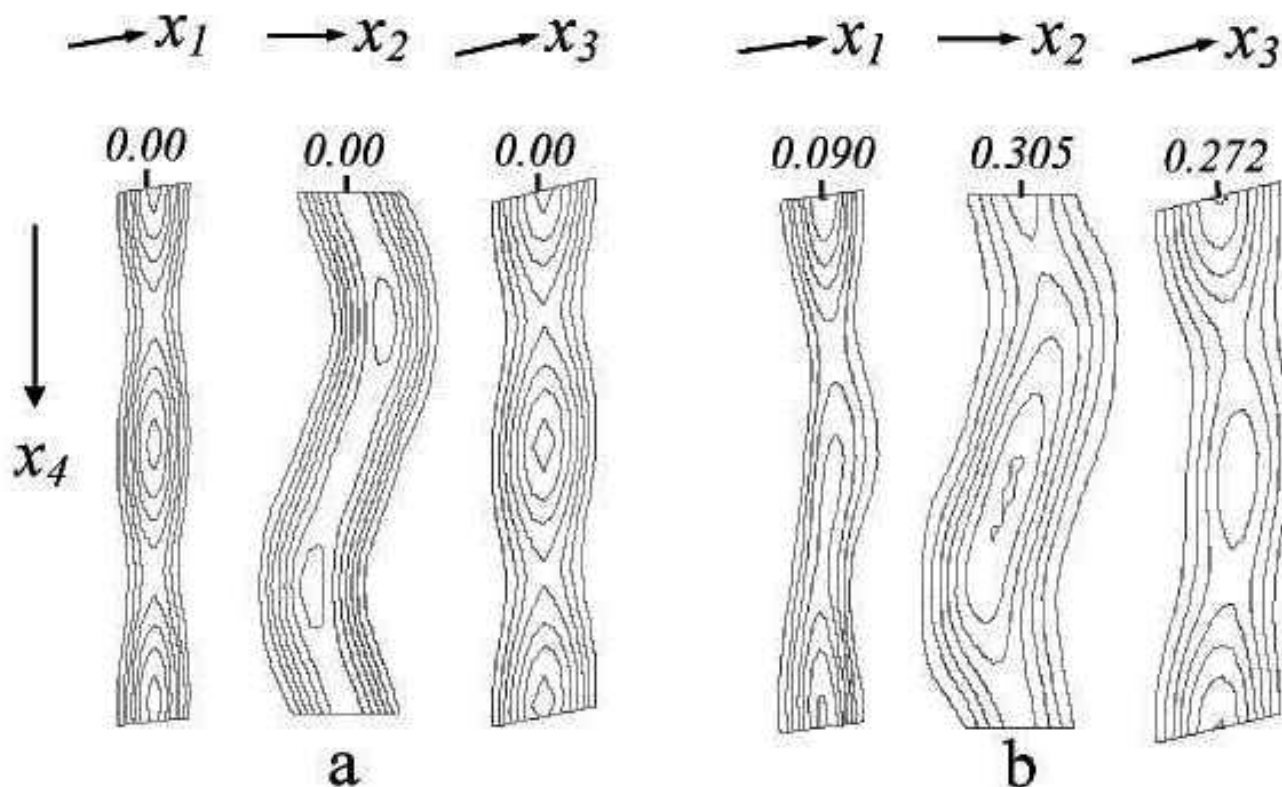
Sections of the 4D electron density map of \gamma - \text{Na}_2\text{CO}_3 . (a) Sections through the average position of the Na atom; (b) Sections through the O (1,3) atom.
